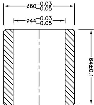
LOCK BUSH (PART NO.—64.08.5051)
