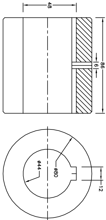
BUSH (PART NO.—64.08.5048)
