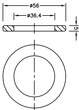
MACHINED WASHER (PART NO.—36DIN125)
